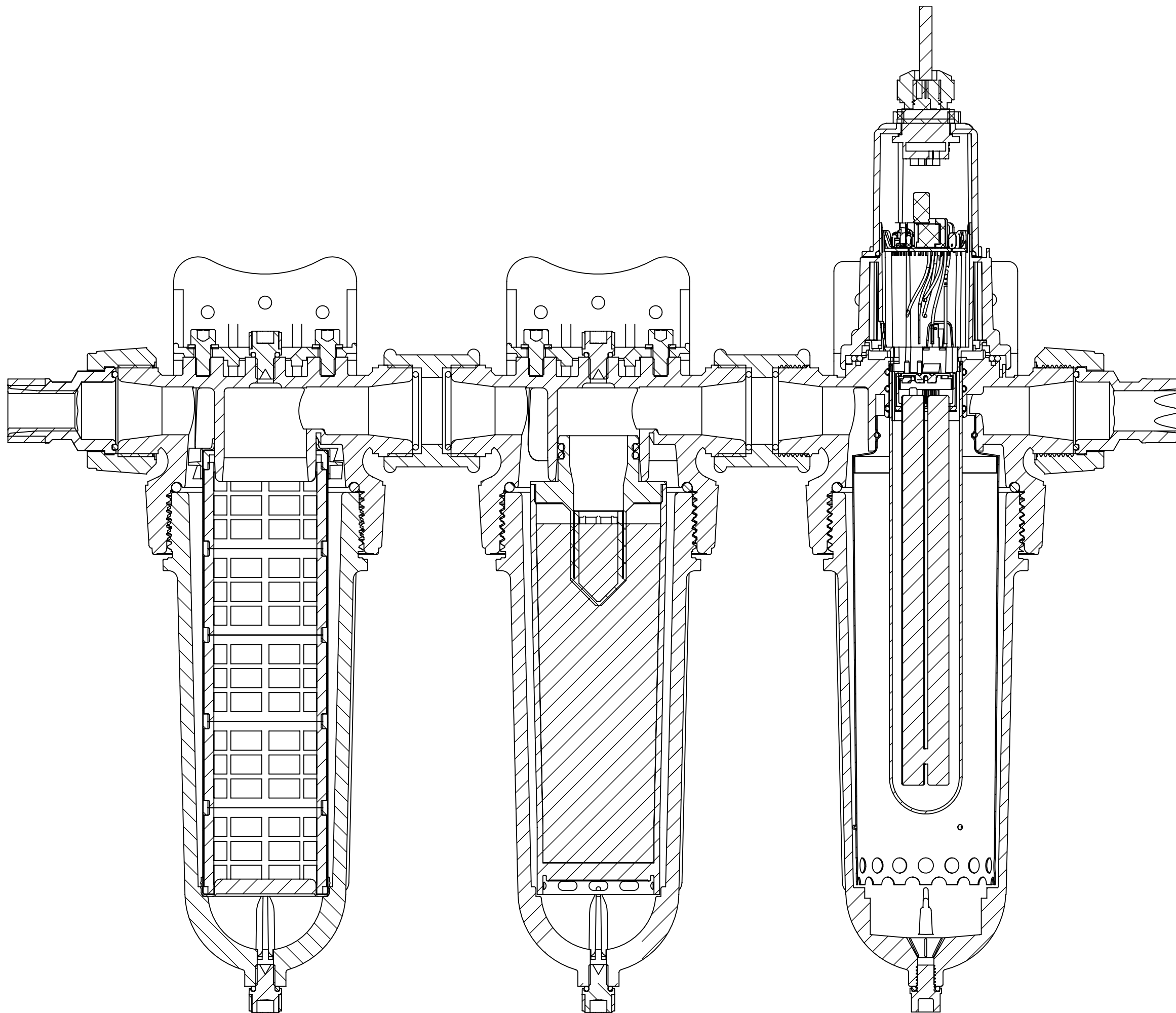
Trio-UV-4100 COUPE
